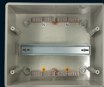
100A RATED ASSEMBLY WITH NEUTRAL & EARTH BARS Suits domestic & commercial installs.
