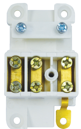
HYJB3TE (Inside view showing Earth Tab)
